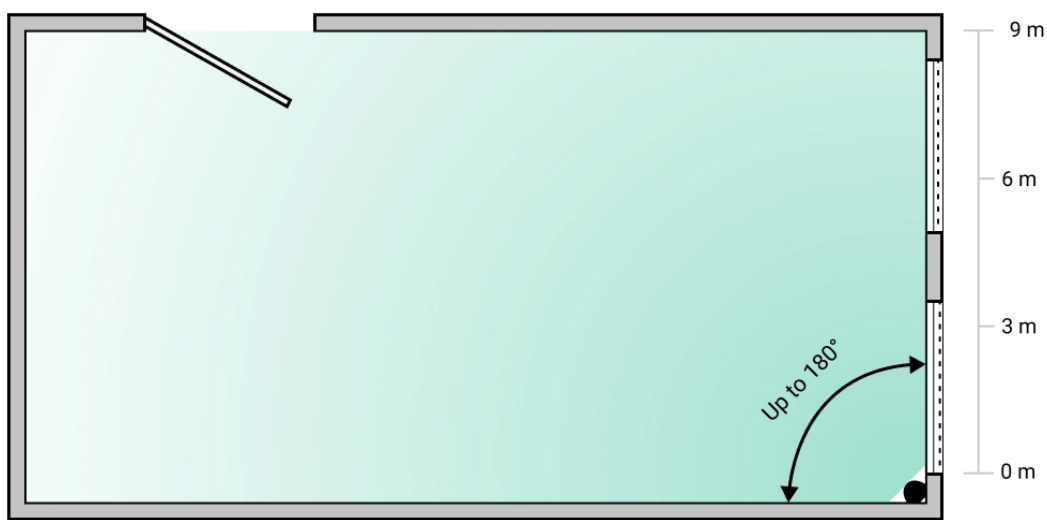
Detection angle of the glass break detector
